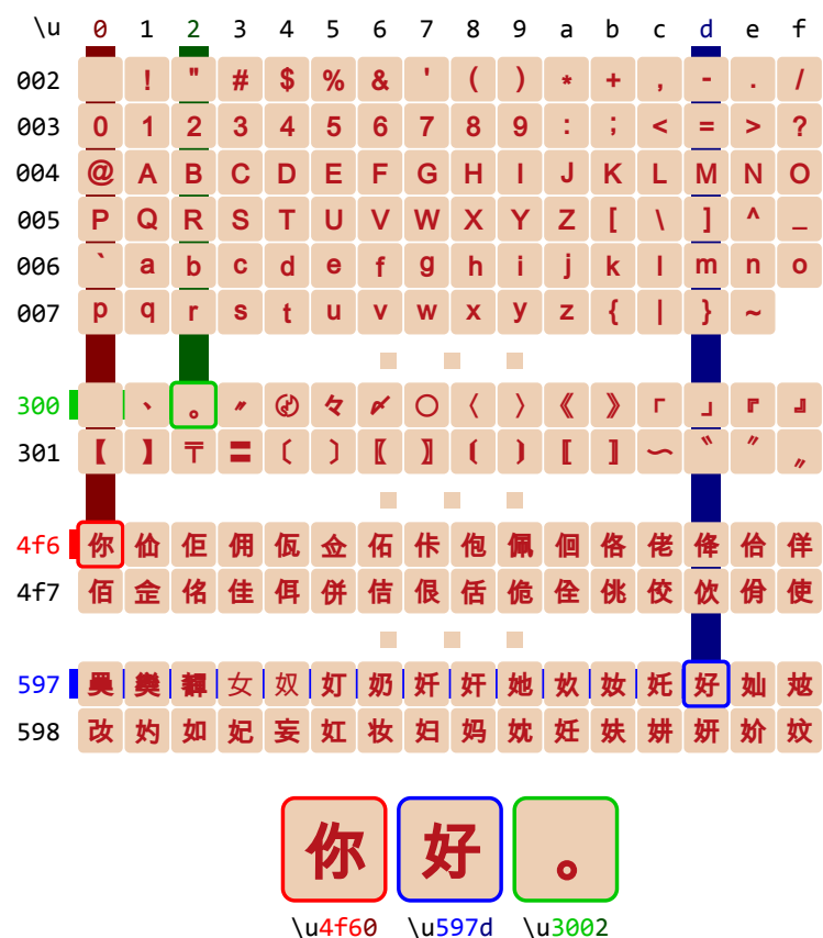
Figure 3.14: A subset of the Unicode character table including the Basic Lating characters as well as some Simplified Chinese characters (简体中文) [489].
